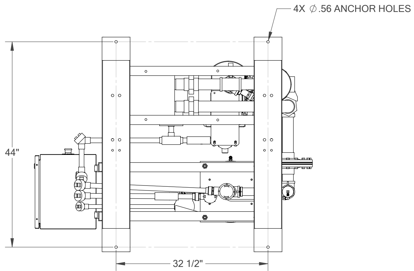
BOTTOM VIEW - ANCHOR HOLE LOCATIONS
