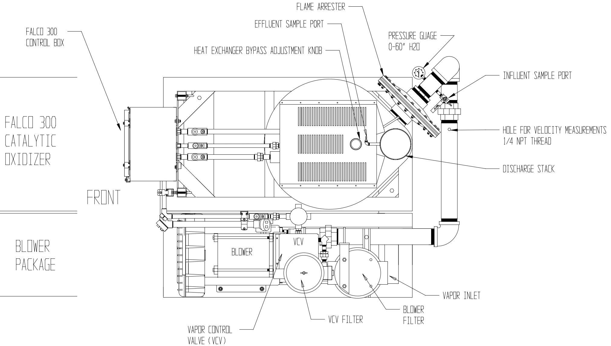
FIGURE 4 FALCO 300 WITH 10 H.P. BLOWER PACKAGE CONTROLS FOR OPERATION
