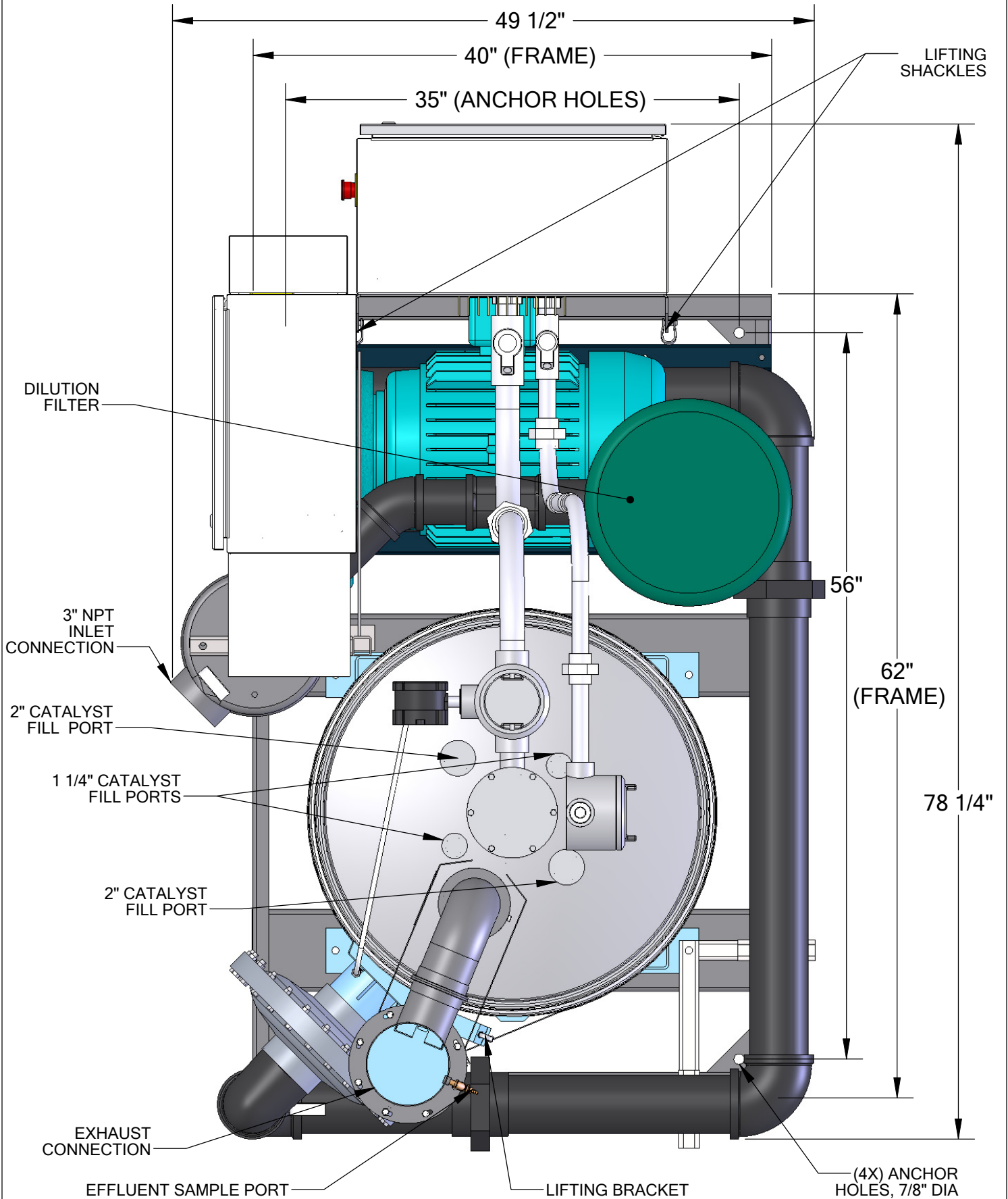
FIGURE 2B: FALCO 600 with VFD- TOP VIEW
