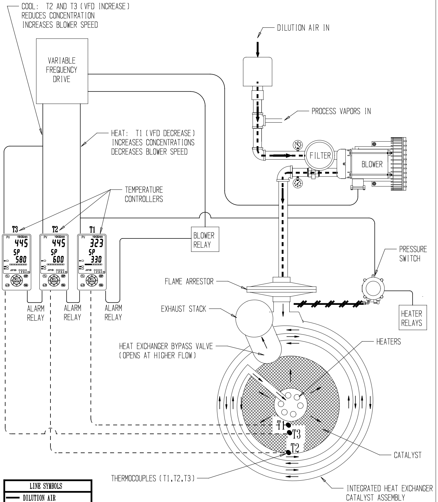
FIGURE 3B: FALCO 600 VFD FLOW AND CONTROL
