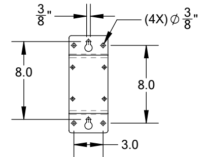
MOUNTING BRACKET DETAIL
