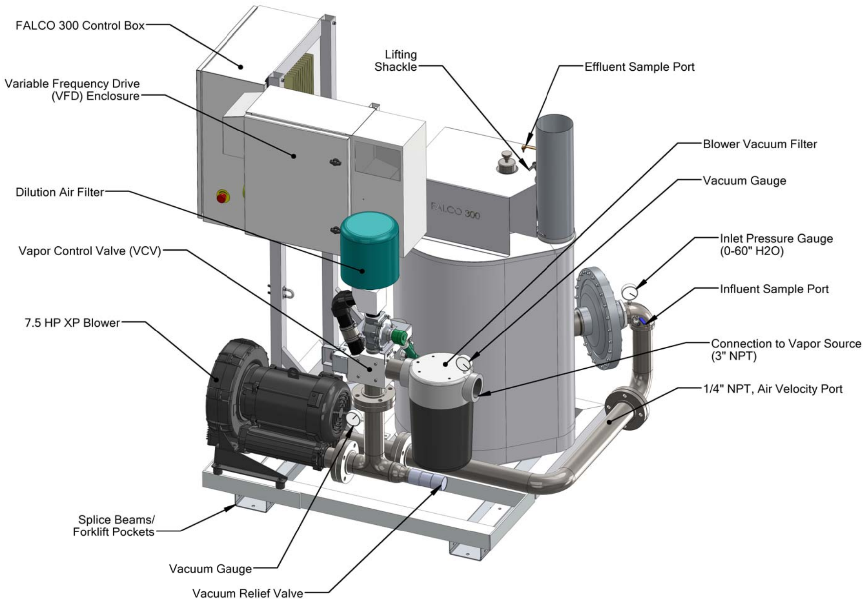
FIGURE 3: FALCO 300 with Regenerative SVE Blower and VFD Major Components / Controls for Operation
